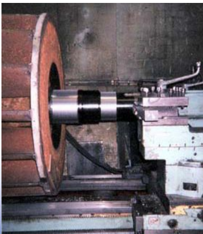
Metallise & grind bearing & seal areas.
