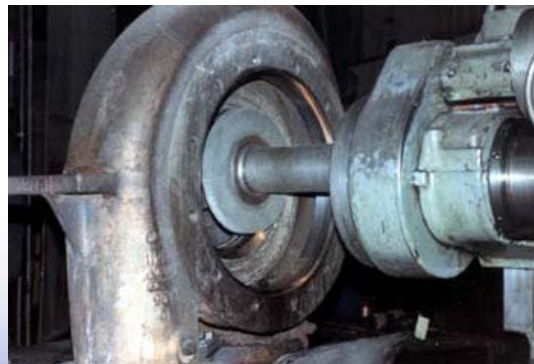
Metallise & grind wear ring seats.
